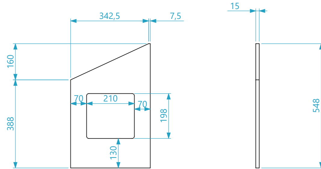
Divisoria x2
