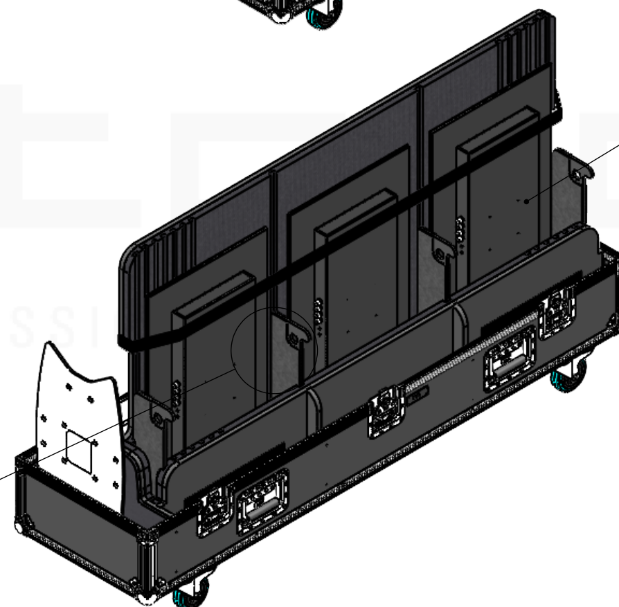
D01.04510.03 Dividers to secure the displays and prevent them from moving side to side.
