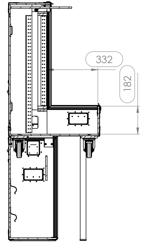
SECTION B-B
