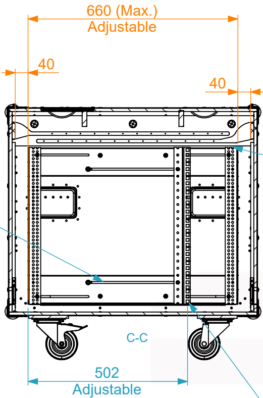
Slots allow additional device support kit
