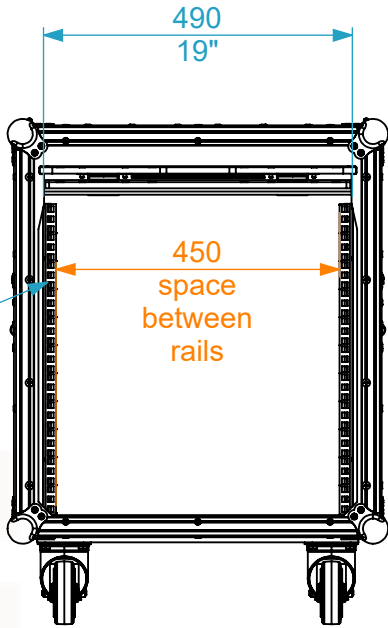
11U (front and rear)
