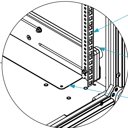
Rack shelf support
