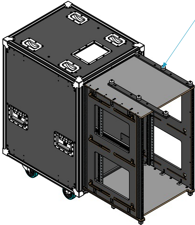
Anti-vibration mounts between the inner rack and the flightcase
