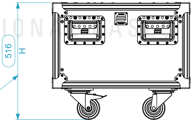
Total height with wheels
