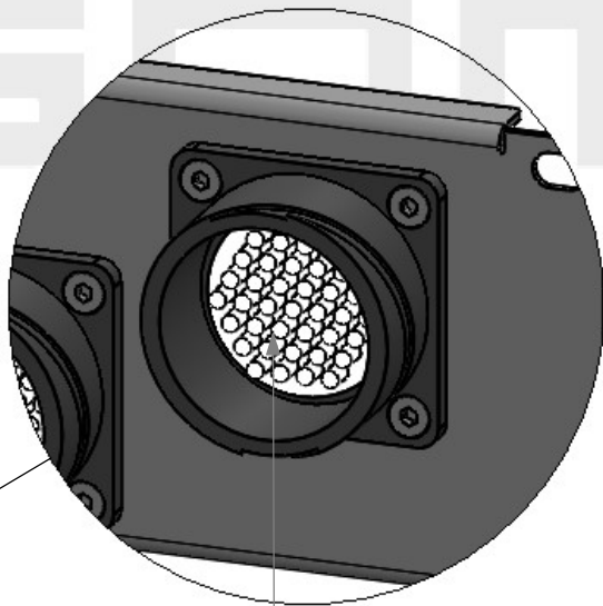
LK 37-pole audio connectors, 12 channels for analog or digital audio transmission
