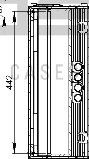
SECTION B-B
