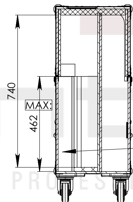
SECTION F-F SCALE 1 : 11
