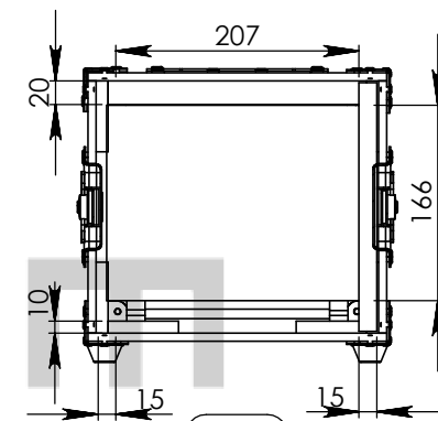
SECTION E-E
