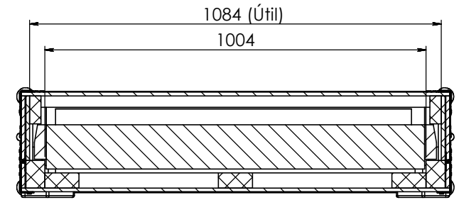
SECTION B-B
