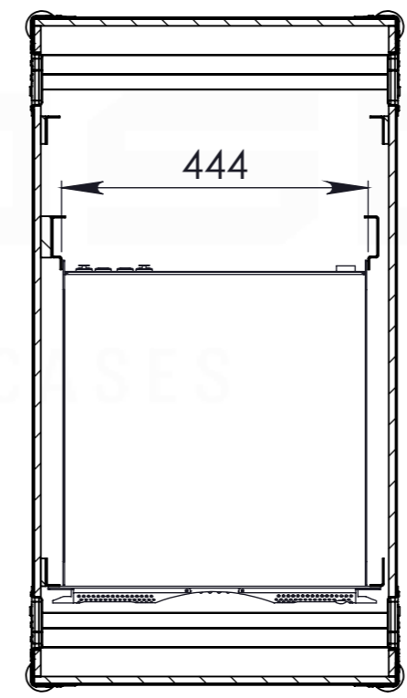
SECTION L-L
