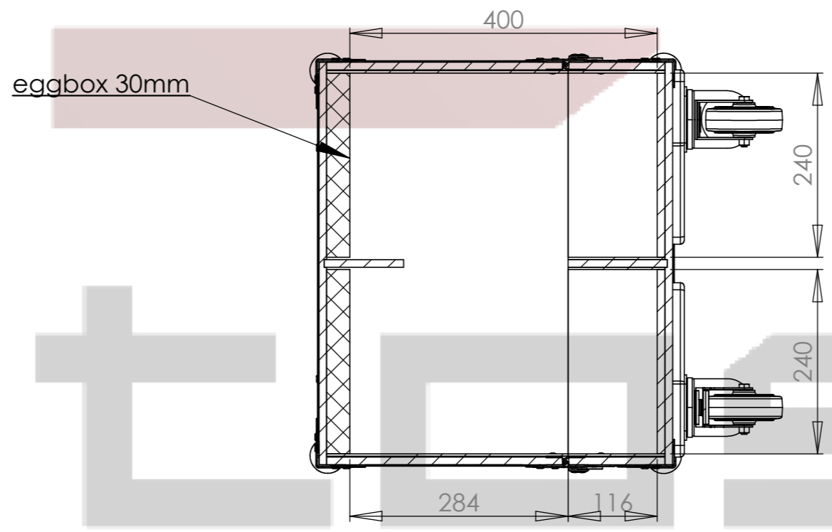
SECTION B-B
