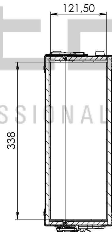
SECTION B-B
