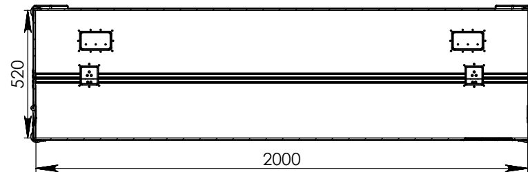
SECTION B-B
