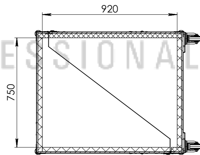
SECTION B-B
