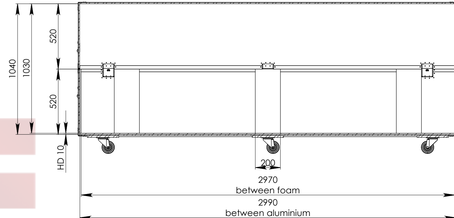
SECTION B-B
