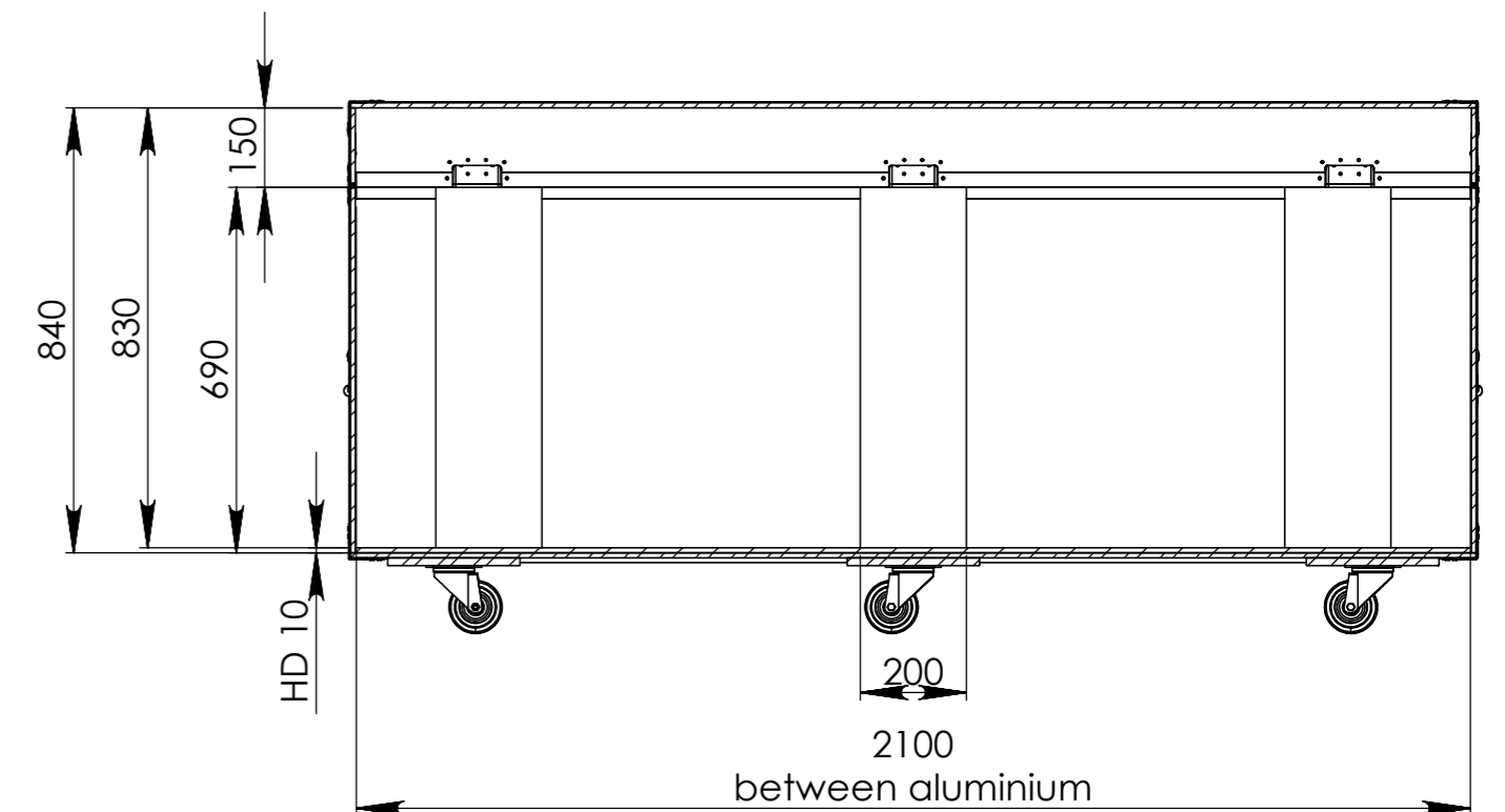
SECTION B-B
